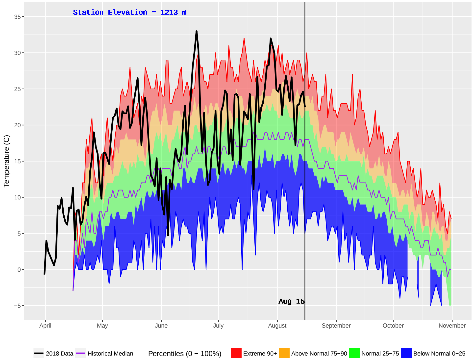
INGENIKA POINT (145) : Historical (1971–2016) and Current (2018) Daily Temperature
