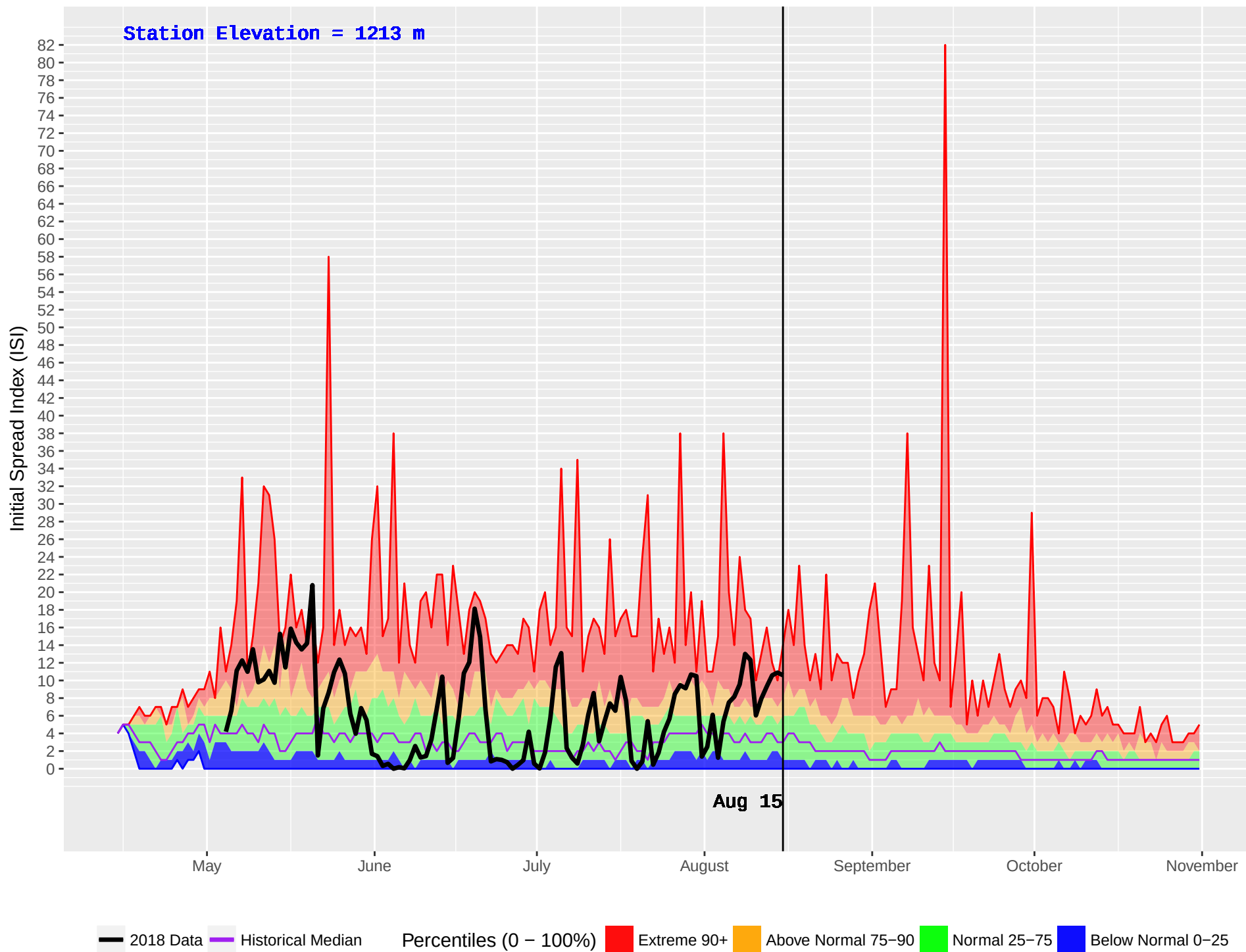
INGENIKA POINT (145) : Historical (1971–2016) and Current (2018) Daily Initial Spread Index (ISI)
